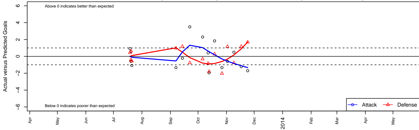
New Millenium FC B95 Dots are actual minus expected GF (blue circles) and GA (red triangles). Blue line is smoothed change in attack strength. Red is smoothed change in defense strength.
